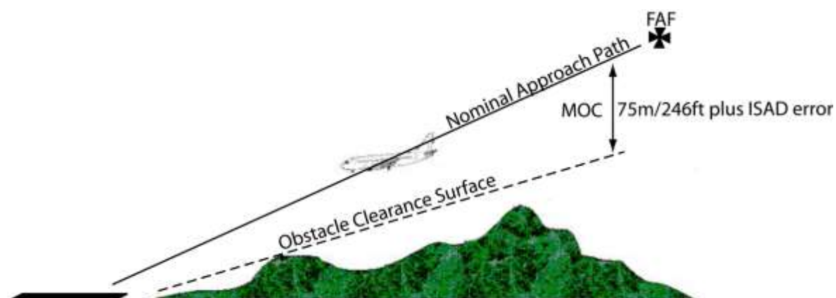
Figure 9.6: Baro-VNAV obstacle clearance for RNP APCH – LNAV
