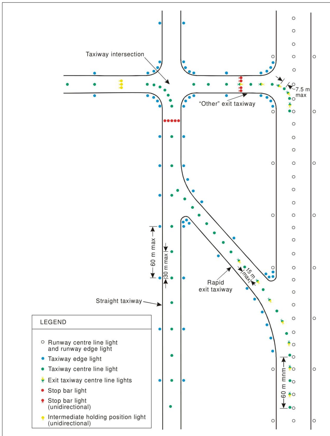
Figure 5-26 Taxiway lighting
