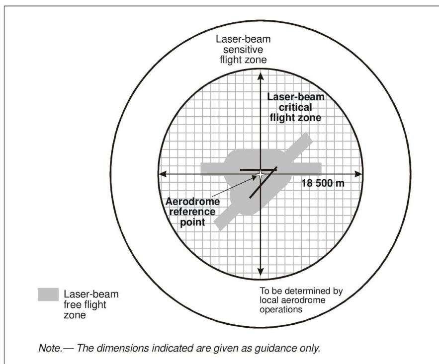
Figure 5-11 Protected flight zones
