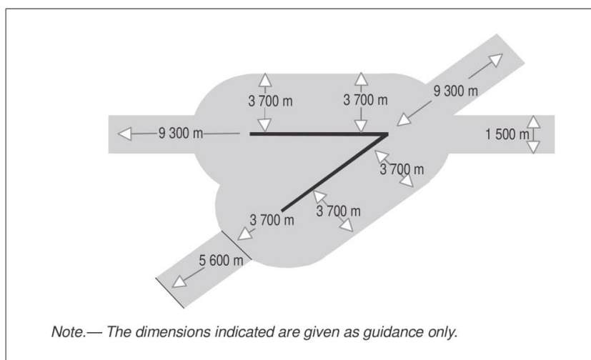
Figure 5-12 Multiple runway laser-beam free flight zone
