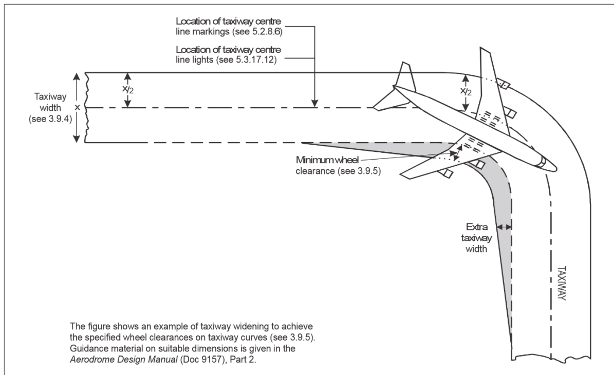
Figure 3-2 Taxiway curve
