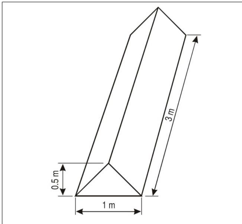
Figure 5-34 Boundary markers.
