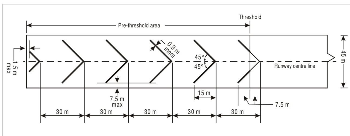
Figure 7-2 Pre-threshold marking
