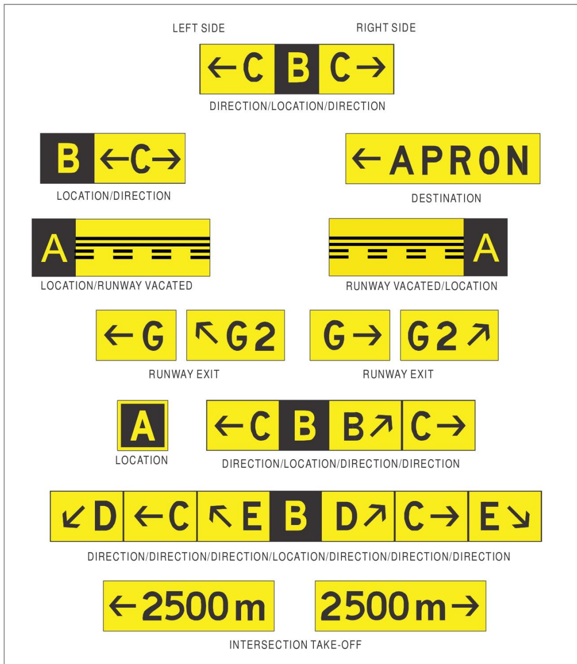
Figure 5-31 Information signs
