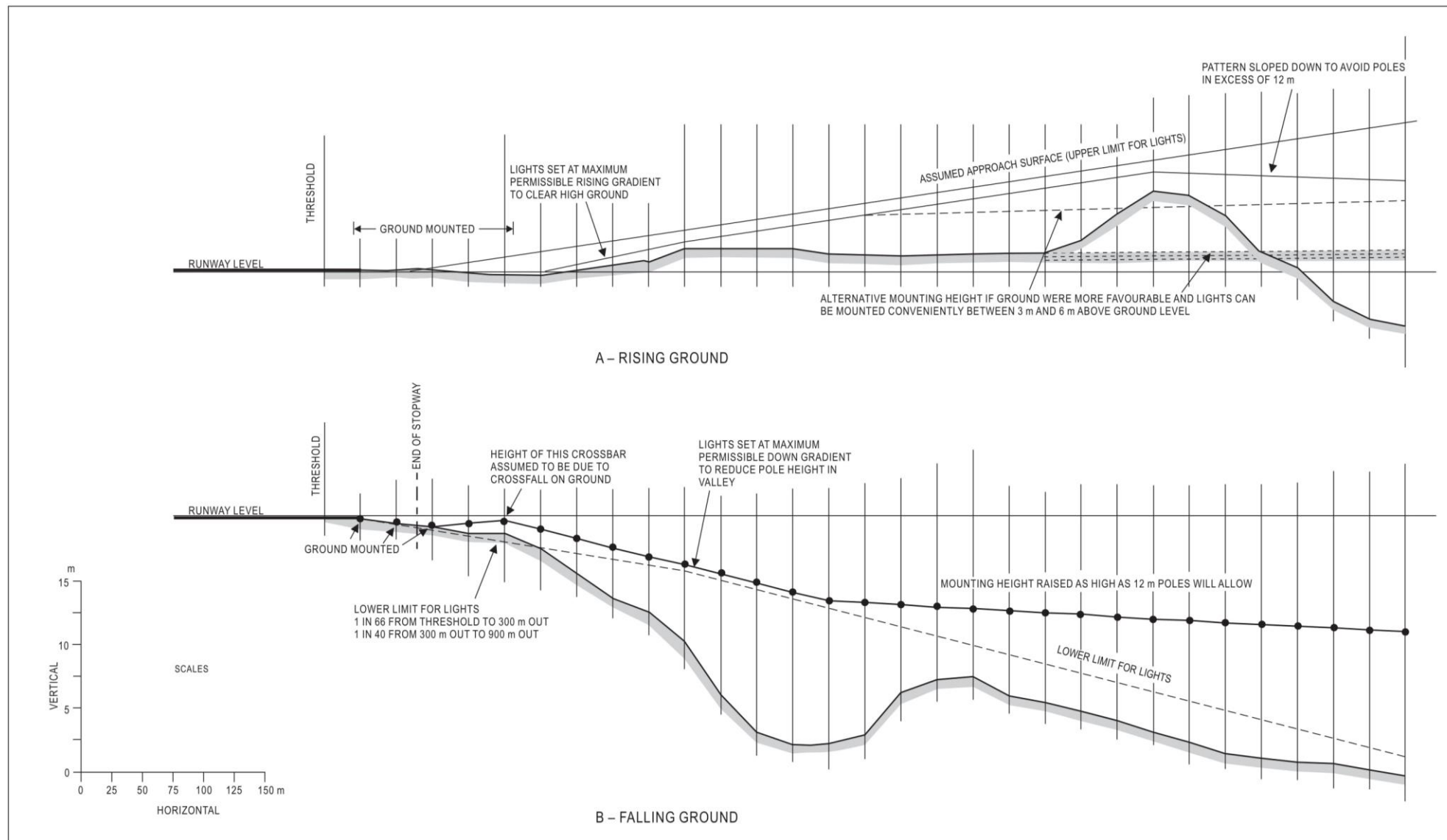
Figure A-9 Vertical installation tolerance
