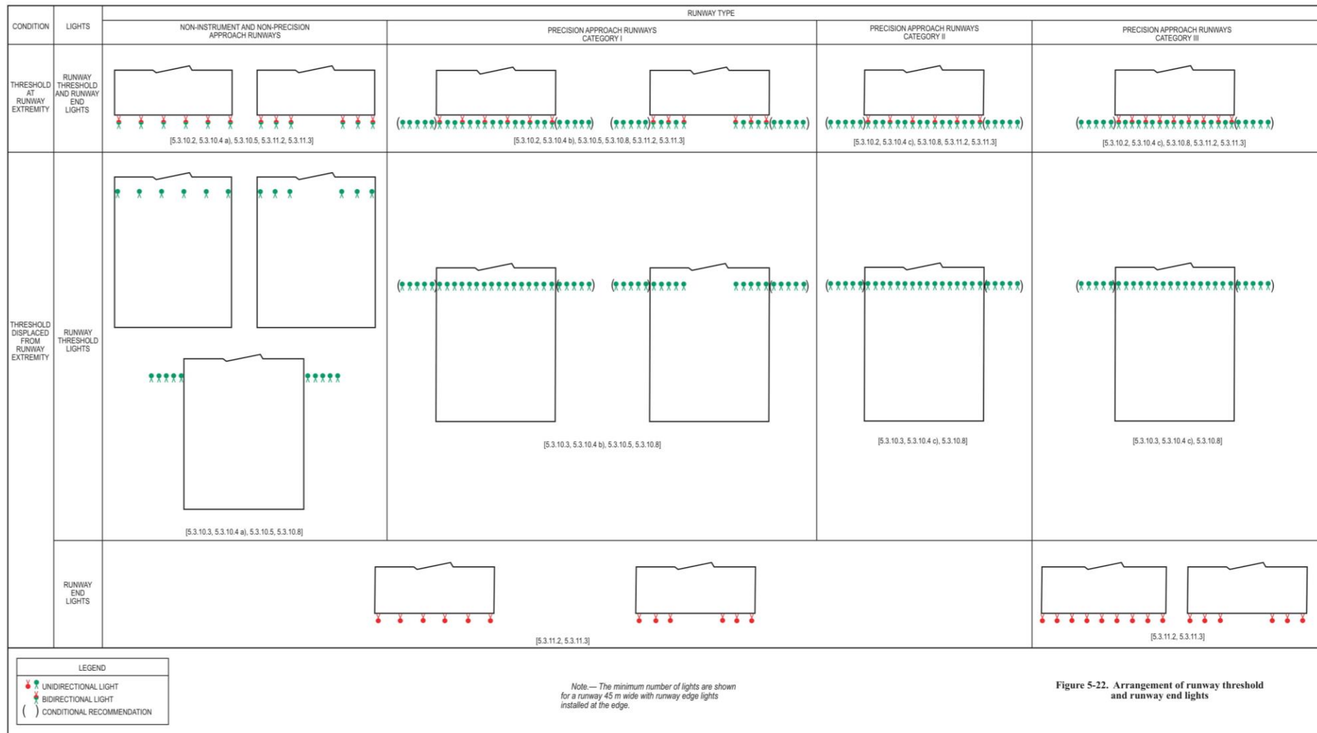
Figure 5-22. Arrangement of runway threshold and runway end lights
