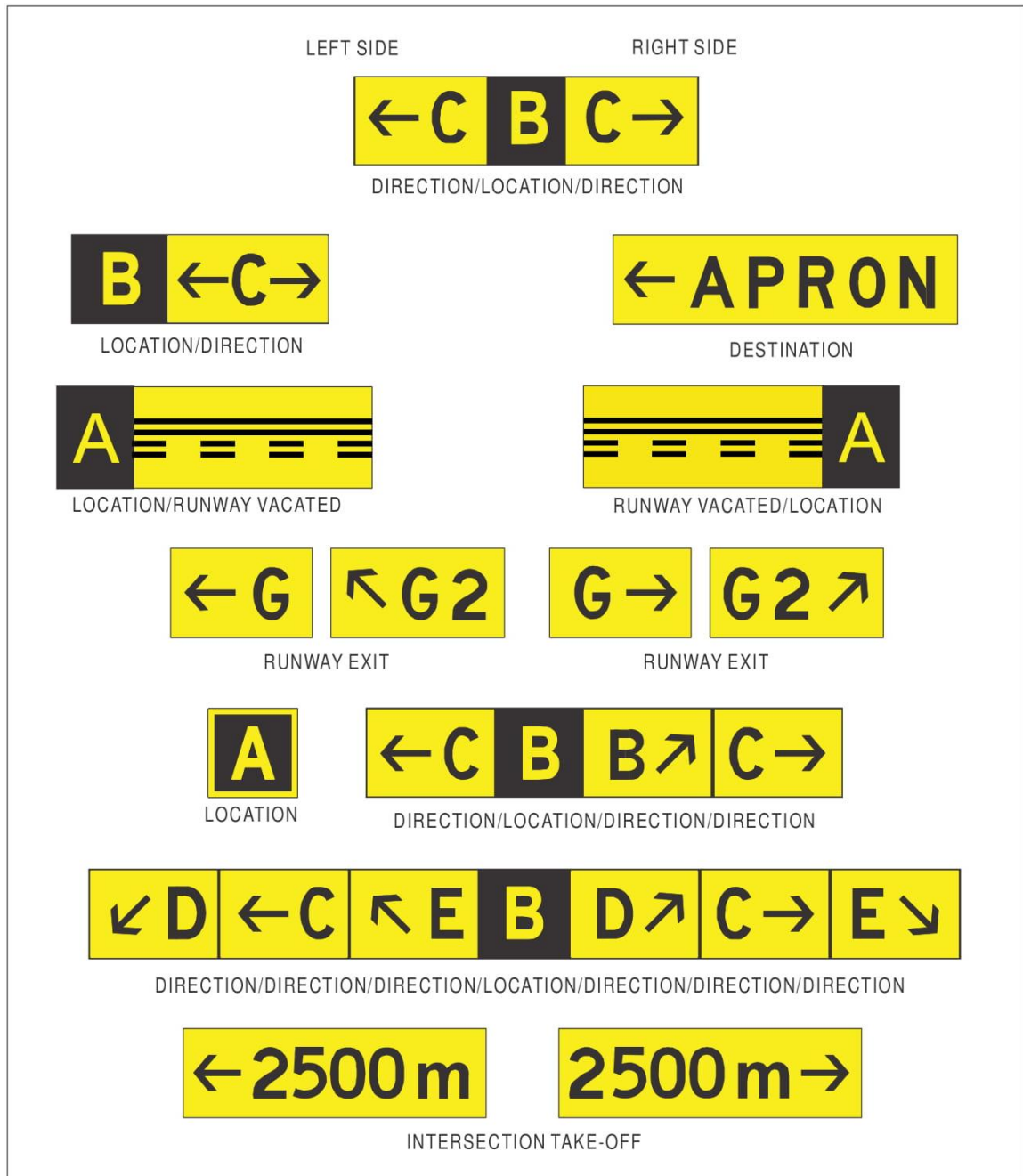
Figure 5-31 Information signs
