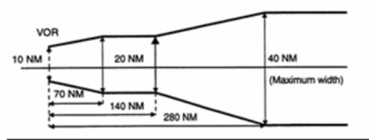
Figure 1: Corridor width from a VOR station
