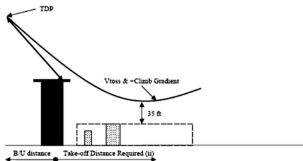
Figure 4: Elevate Helipad take – off
