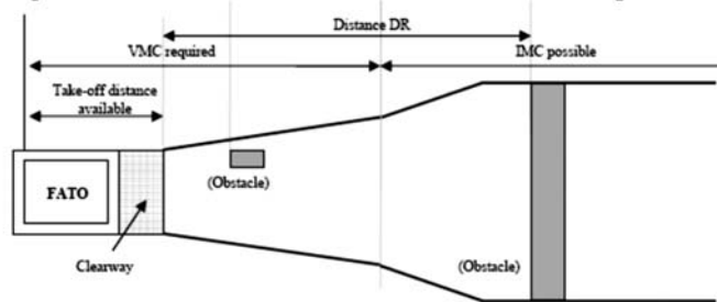
Figure 4: Performance Class 2 Obstacle Clearance (plan view)
