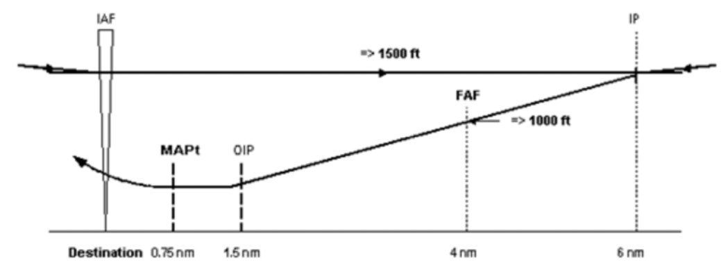
Figure 4: Vertical profile
