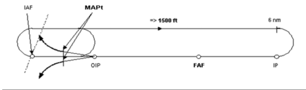
Figure 3: Holding pattern & race track procedure
