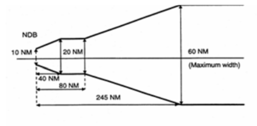
Figure 2: Corridor width from an NDB
