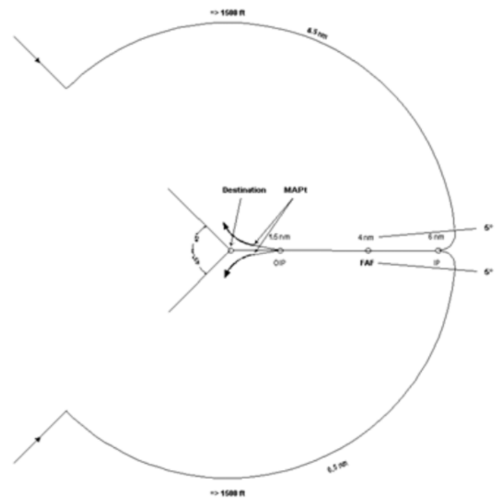
Figure 1: Arc procedure
