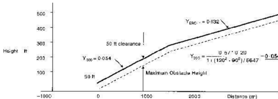
Figure 1: Assumed engine failure height 300 ft
