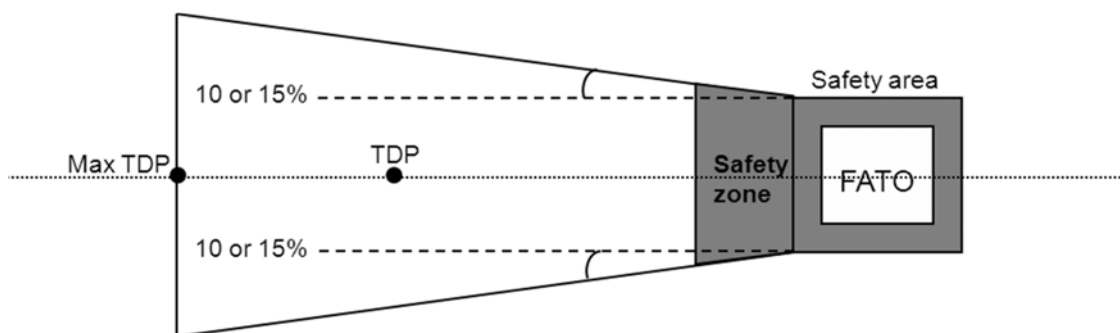
Figure 2: Obstacle accountability
