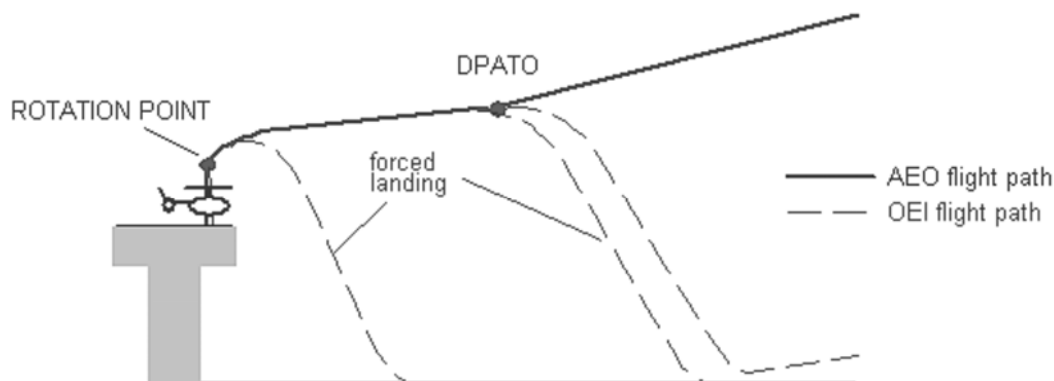
Figure 1: Take-off profile
