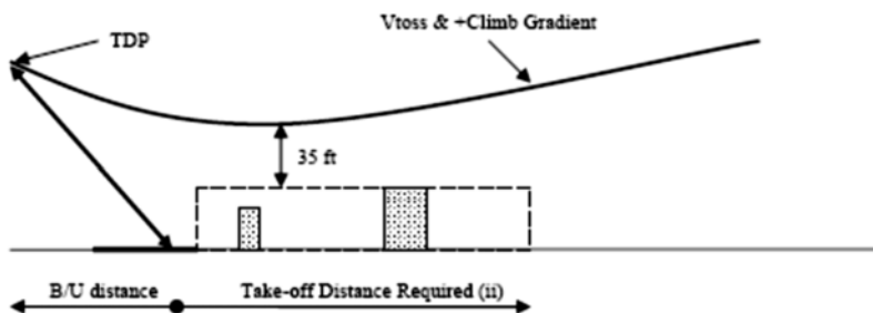
Figure 3: Helipad take-off
