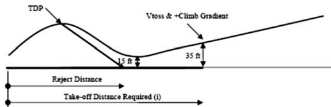
Figure 1: Clear Area take – off
