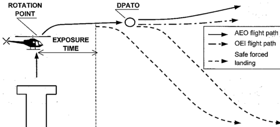
Figure 2: Typical take-off profile PC2 from a helideck/elevated FATO with exposure time, non-hostile environment
