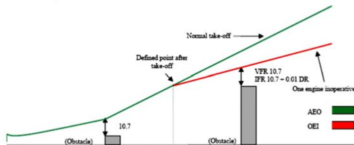
Figure 3: Performance Class 2 Obstacle Clearance
