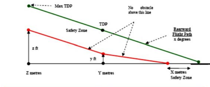
Figure 1: Rearward flight path
