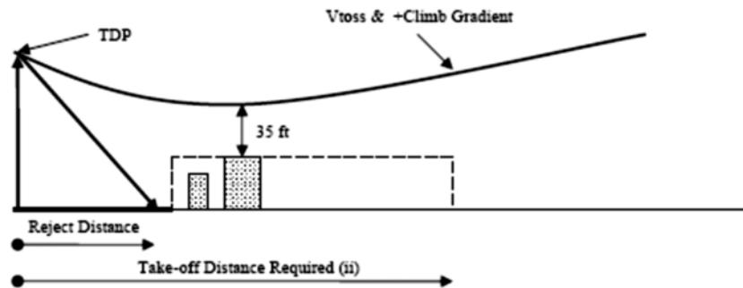
Figure 2: Short Field take-off
