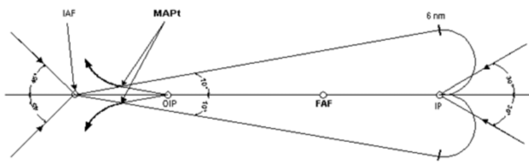
Figure 2: Base turn procedure – direct approach
